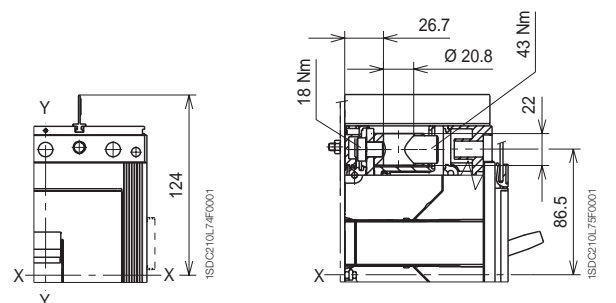
Front for copper/aluminum cables - 1x240 mm 2
